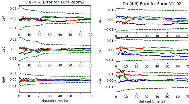
Fig. 15: Evaluation of the proposed system for \mathbf{D}_a with tum_room1 (left) and EuRoc V1_02 (right) trajectories using \text{imu2}\{\mathbf{D}_{w6}, \mathbf{D}_{a6}, {}^I\mathbf{R}\} . 3\sigma (dotted lines) and estimation errors (solid lines) for four different runs (different colors) are drawn. The convergence of d_{a4} , d_{a5} and d_{a6} is poor for the EuRoc V1_02 due to lack of motion excitation.
