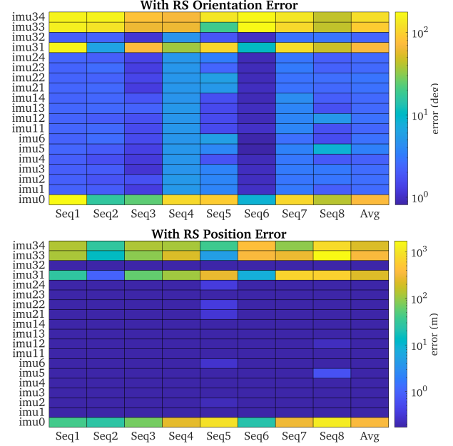
Fig. 11: Results on TUM RS VIO Dataset with readout time calibration, with different IMU intrinsic models. The averaged absolute trajectory errors (ATE) of 5 runs in degree (top) and meters (bottom) are provided. Note that camera intrinsics, and IMU-camera spatial-temporal parameters are calibrated.
