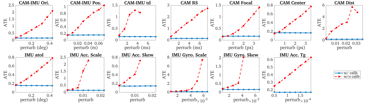
Fig. 4: Absolute trajectory errors (ATE) using \text{imu22}\{\mathbf{D}_{w6}, \mathbf{D}_{a6}, {}^I\mathbf{R}, \mathbf{T}_{g9}\} and radtan on the tum_corridor with full 3D motion given different levels of perturbation. Only the calibrated parameter was perturbed while other parameters were initialized to their true values and not estimated. ATE above eight meters were not reported and can be considered as divergence.
