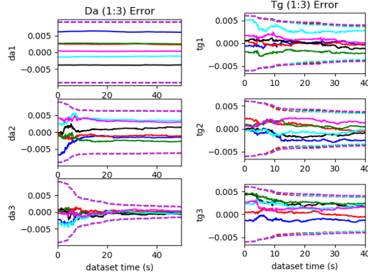
Fig. 6: Evaluation on the sine_3d with constant acceleration along x-axis using \text{imu22}\{\mathbf{D}_{w6}, \mathbf{D}_{a6}, {}^I\mathbf{R}, \mathbf{T}_{g9}\} . The estimation errors and 3\sigma bounds for d_{a1} , pitch and yaw of {}^I\mathbf{R} cannot converge. Note that t_{g1} , t_{g2} and t_{g3} also converge very slow.
