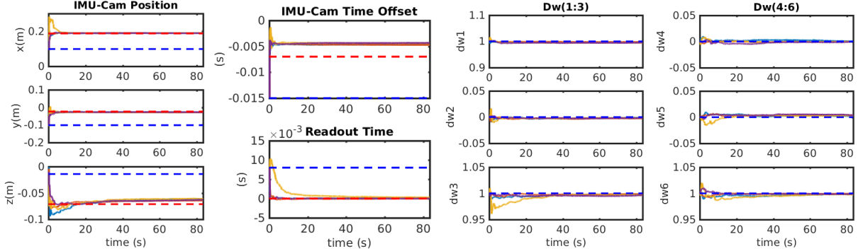
Fig. 17: Calibration results (from four 3D-motion datasets in Section X with colored solid lines) for {}^C\mathbf{p}_I , t_d , t_r and \mathbf{D}_w of the proposed system evaluated using \text{imu2}\{\mathbf{D}_{w6}, \mathbf{D}_{a6}, {}^I\mathbf{R}\} and equidist . Red and blue dotted lines denote the reference value from Kalibr and initial (perturbed) values, respectively.
