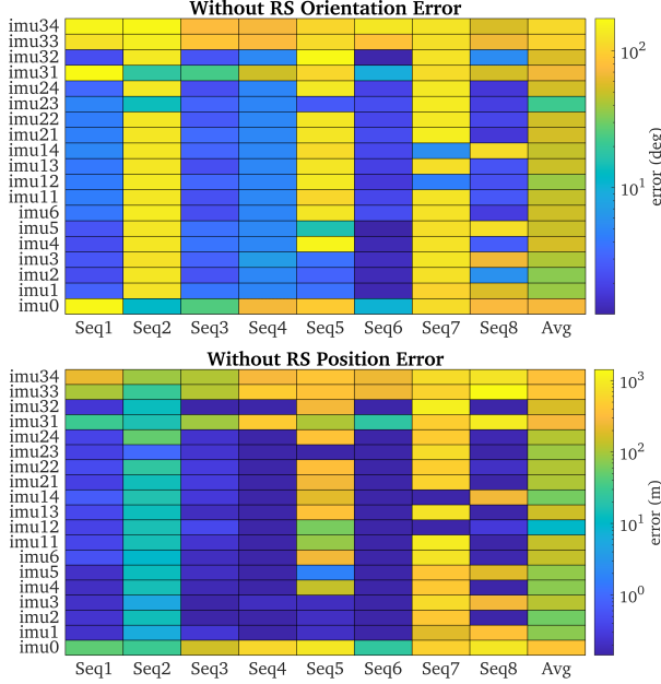
Fig. 10: Results on TUM RS VIO Dataset without readout time calibration, with different IMU intrinsic models. The averaged absolute trajectory errors (ATE) of 5 runs in degree (top) and meters (bottom) are provided. Note that the camera intrinsics, and IMU-camera spatial-temporal parameters are calibrated.
