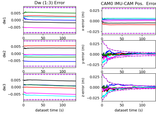
Fig. 5: Evaluation on tum_room with one-axis rotation using \text{imu22}\{\mathbf{D}_{w6}, \mathbf{D}_{a6}, {}^I\mathbf{R}, \mathbf{T}_{g9}\} . Note that the estimation errors and 3\sigma bounds for d_{w1} , d_{w2} , d_{w3} and the IMU-camera position calibration along the rotation axis can not converge.
