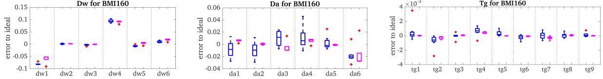
Fig. 9: IMU intrinsic evaluation of Bosch BMI160 IMU used in TUM Rolling Shutter VIO datasets using the proposed method (blue, left) and Kalibr (magenta, right) relative to the “ideal” sensor intrinsics. Red + denotes outliers.
